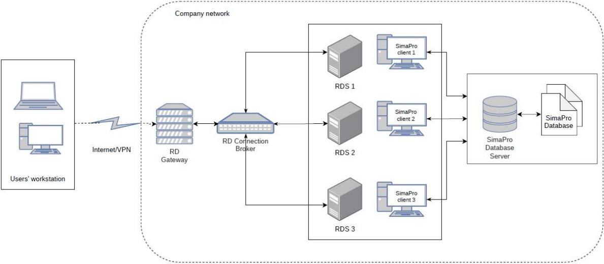
Figure 3 Example (2) of the recommended SimaPro setup. With this setup you have several installations of remote desktop server with the SimaPro client, all connecting to the same SimaPro database server.
