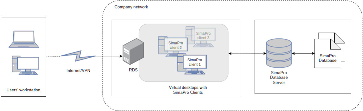
Figure 2 Example (1) of the recommended SimaPro setup. With this setup, you connect to the remote desktop where several instances of SimaPro client are run and connected to the SimaPro database server.
