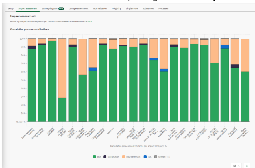
Figure 36: Calculation results
