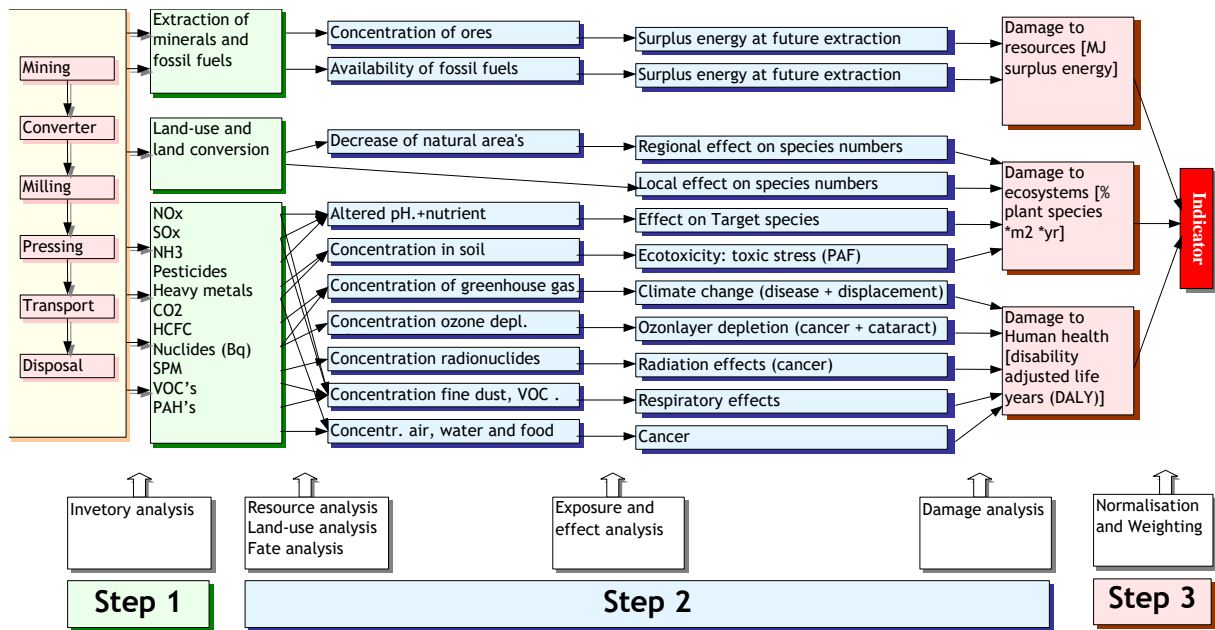
Figure 5: Detailed representation of the damage model
